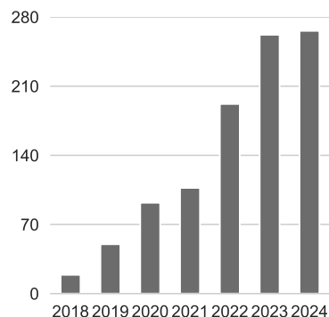
Citation Trend (Scholar)
